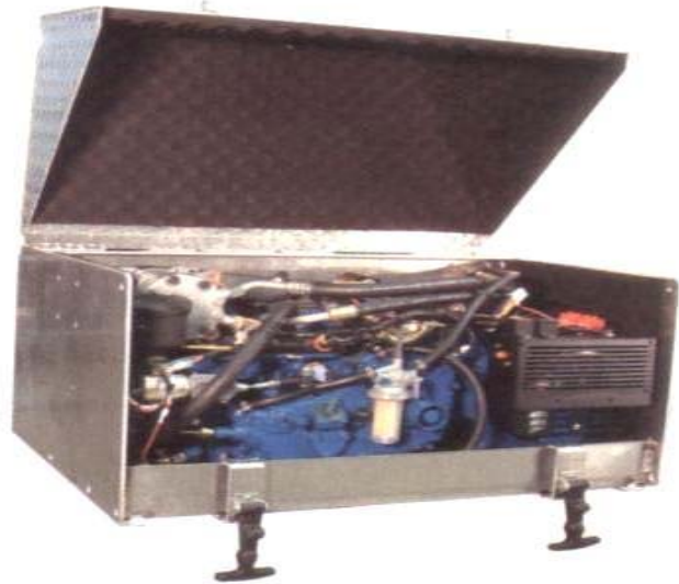
Alliance Custom Premium Auxiliary Power Unit System w/ 3.5kw Generator Specifications: (Provides 3500 Watts of 110 Volt Electricity)
